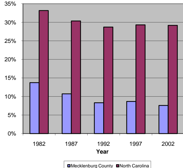
Percent Farmland
